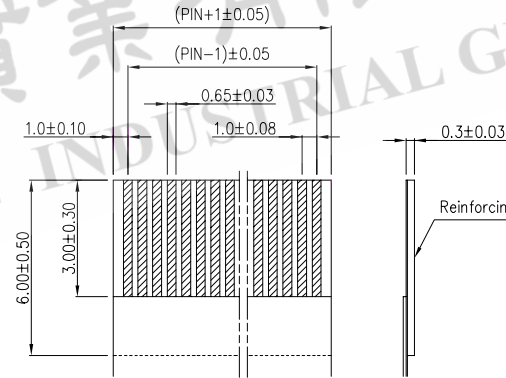
RECOMMENDED FFC/FPC DIM.
