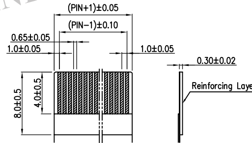
RECOMMENDED FFC/FPC DIM.
